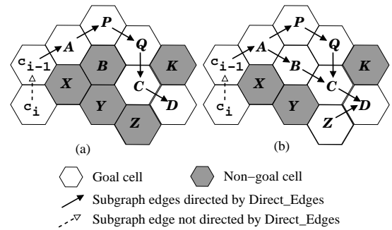
Fig. 9. Snapshots of DIRECT_EDGES execution depicting: (a) a situation in which a vertical edge is not added to H due to violation of Definition 3, part 2(b), and (b) a situation in which a vertical edge is not added to H due to violation of Definition 3, part 2(a). Initial undirected edges not shown.
