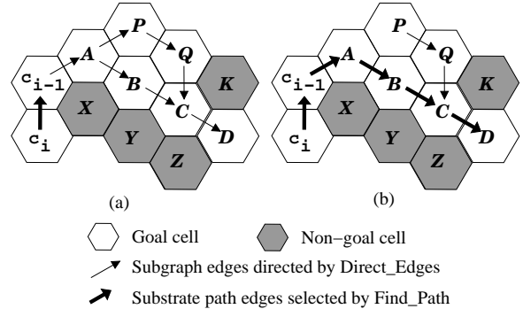
Fig. 8. Snapshots of FIND_PATH execution, (a) before and (b) after edge (c_i, c_{i-1}) is added to the substrate path.
