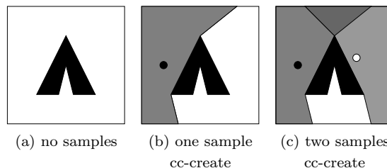
Figure 1: (a) A two-dimensional environment with a polygonal obstacle. (b) One sample is added. (c) One more sample is added. Note that the coverage of the two samples overlaps above the obstacle.
