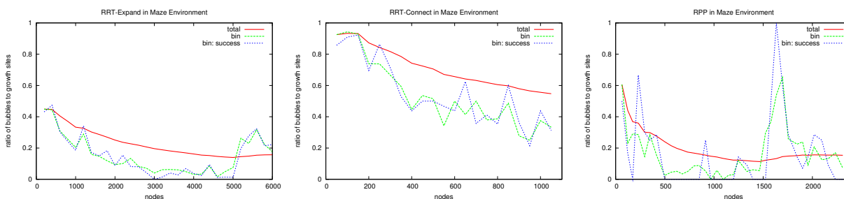
Figure 6: Global metrics for maze environment mapped with RRT-Expand (left), RRT-Connect (center), and RPP (right). For each sampler we show the total ratio of bubbles to growth sites (total), the bin ratio of bubbles to growth sites (bin), and the bin ratio of bubbles to growth sites from successful expansions (bin: success) with bins of either 200 nodes
