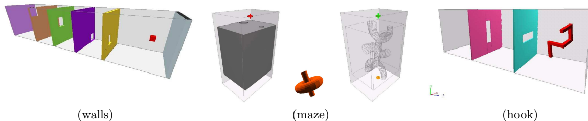
Figure 4: ( walls ) 6-DOF cubic robot, four short passages; ( maze ) solid view, 6-DOF robot, and wire view; ( hook ) 6-DOF hook robot, two medium passages.
