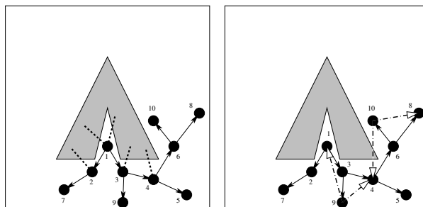
Figure 3: Incremental model of the problem in Figure 1. Numbers indicate vertices and their placement order. Solid arrows indicate successful connections and their direction (a) Dotted lines indicate failure growth attempts from the source node. (b) Hollow arrows indicate connection attempts for the expansion ratio test when nodes 9 and 10 were added to the model.
