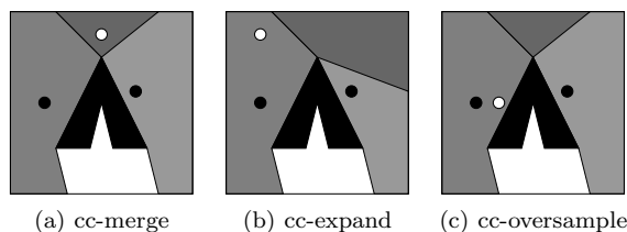
Figure 2: New samples (hollow dots) are added. (a) A cc-merge sample falls in the intersecting coverage of the two existing samples connecting the two regions. (b) A cc-expand sample increases the coverage of the component to the left, but does not change the connectivity. (c) Oversampling does not increase coverage or connectivity.
