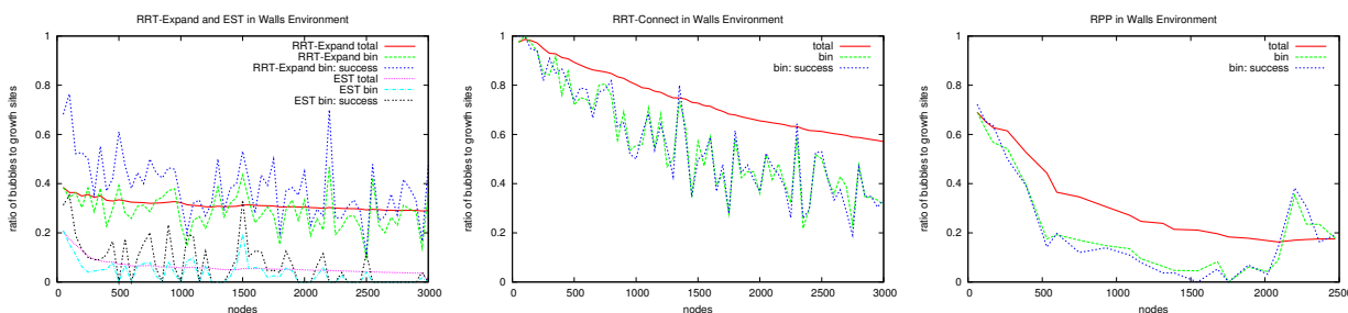
Figure 5: Global metrics for walls environment mapped with RRT-Expand (left), EST (left), RRT-Connect (center), and RPP (right). For each sampler we show the total ratio of bubbles to growth sites (total), the bin ratio of bubbles to growth sites (bin), and the bin ratio of bubbles to growth sites from successful expansions (bin: success) with bins of either 50 or 200 nodes
