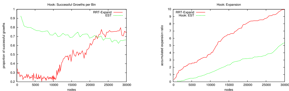
Figure 7: Results for hook environment mapped with RRT-Expand and EST. We show the proportion of successful growths per bin and the accumulated expansion ratio with bins of 50 nodes
