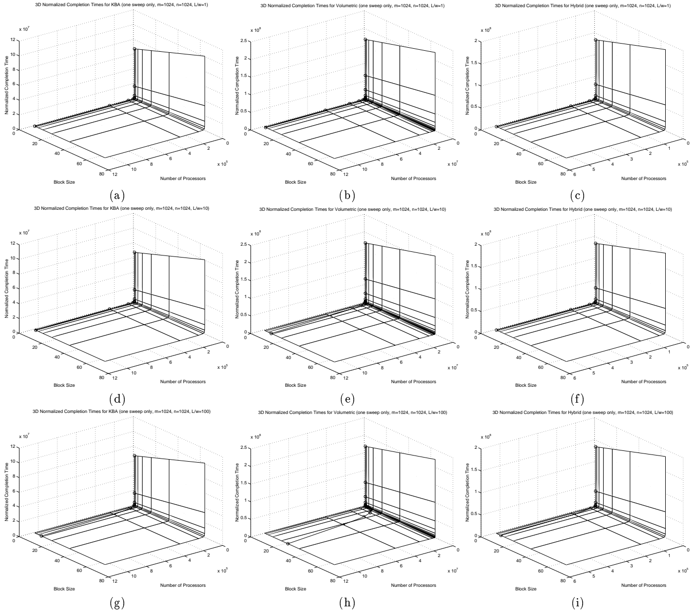
Figure 4: These 3D surfaces demonstrate the effect of the block size parameter k on the normalized completion times of KBA ((a), (d), and (g)), Volumetric ((b), (e), and (h)), and Hybrid ((c), (f), and (i)). These plots are for a single sweep in a cubic three-dimensional spatial domain ( m = n = h = 1024 ) over 1 \leq k \leq 64 . We look at three different cases of the machine parameter L/\omega , representing machines where communication is relatively inexpensive ( L/\omega = 1 , (a-c)), communication is moderately expensive ( L/\omega = 10 , (d-f)), and communication is relatively expensive ( L/\omega = 100 , (g-i)). The normalized completion times obtained using k_{opt} are traced out as lines on the 3D surfaces.
