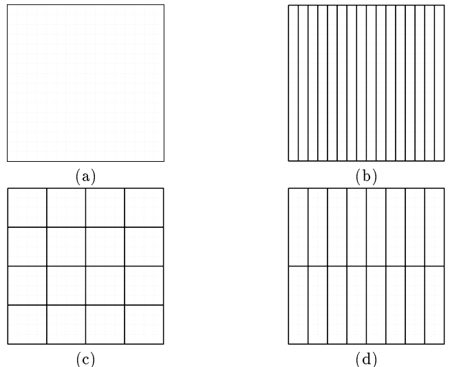
Figure 2: Figure (a) is a diagram of an example two-dimensional base grid ( m = n = 16 ). Figures (b), (c), and (d) demonstrate how KBA ( \phi_m = 1, \phi_n = 16 ), Volumetric ( \phi_m = \phi_n = 4 ), and Hybrid ( \phi_m = 2, \phi_n = 8 ) partition the base grid shown in (a), given p = 16 processors.
