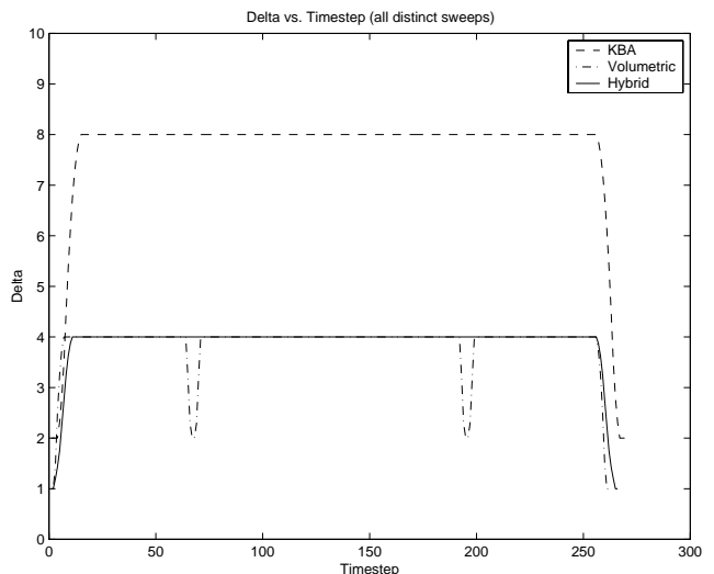
Figure 3: This plot shows values of \delta for the case of all distinct sweeps, one for each octant of directions, in three dimensions. Here we see that KBA typically has a \delta equal to the number of sweeps, while Volumetric and Hybrid typically have \delta values equal to one half of the number of sweeps. This example assumes a representative grid of size m = n = h = 256 with p = 64 processors.
