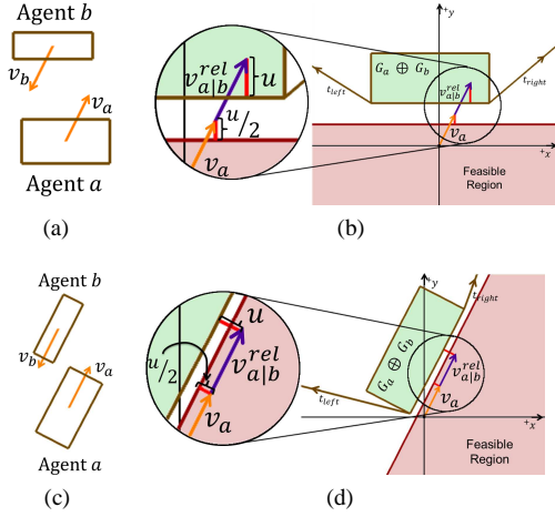
Fig. 2. (a) Two rectangular robots a and b on a collision course. (b) Construction of VO_{a|b}^\tau for the scenario shown in (a). A linear constraint (pink region) on v_a is derived from the velocity obstacle, and it can be seen that v_a does not lie in the feasible region. (c) The same scenario as before, except a and b are rotated. (d) This rotation creates a scenario where v_a is already a feasible velocity for the next timestep.
