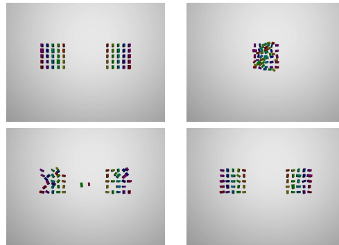
Fig. 5. Progression of the Lines scenario for 50 agents. Agents are positioned in opposing groups of parallel lines of five, and instructed to reach their horizontally-symmetric positions. This scenario requires agents to navigate around many stopped agents with very small gaps between them.
