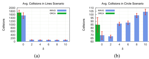
Fig. 11. The number collisions experienced, on average, by those agents who reached their goals in the (a) Lines and (b) Circle scenarios. Agents using RRVO generally do not collide more often on average than if they were to use ORCA, despite RRVO's relaxed collision-avoidance guarantees. In fact, in the Lines scenario they collide significantly less than in ORCA due to deadlocked agents colliding with completed ones.
