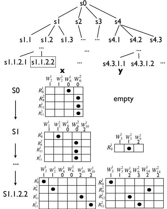
Figure 4: A hierarchical view of seed interleaving generation
